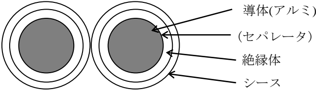
2 心 (AL-CVD)
